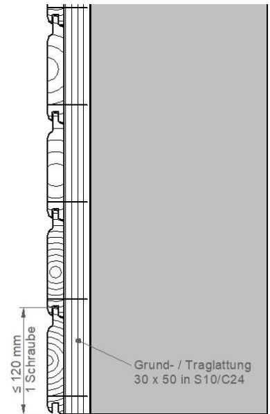
Softline 20 mm N+F
